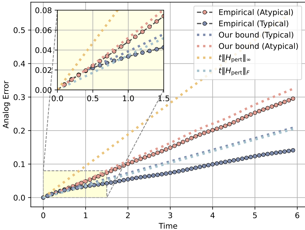
QIMF, long-time evolution with disorder
